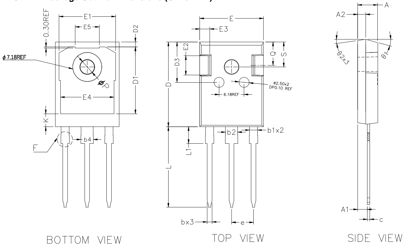
COMMON DIMENSIONS (UNITS OF MEASURE IS mm)
